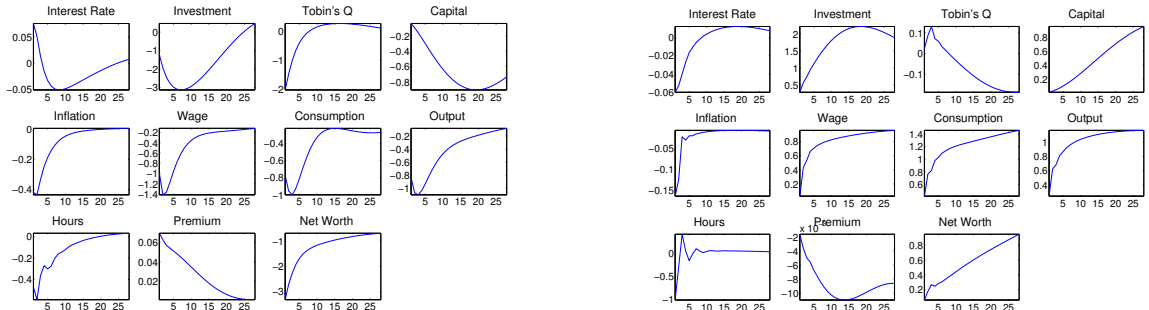
IRFs for a monetary shock
