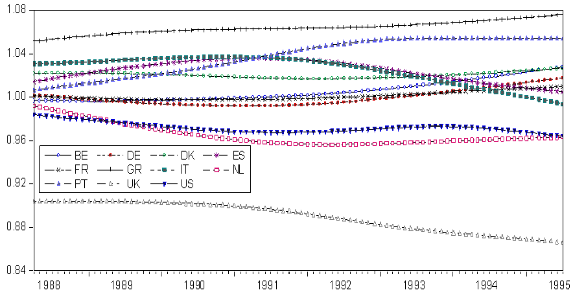
Figure 3: h_{ict} for the U.S. dollar price of i =clothing for each of 11 countries
