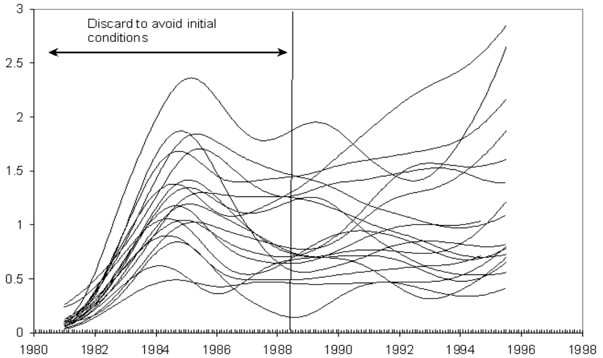
Figure 2: H_{it} for i = 1, \dots, 19 across 12 countries. First half of sample discarded to control for initial conditions. H_{it} = H_{it} = \frac{1}{C} \sum_{c=1}^C (h_{ict} - 1)^2 , where h_{ict} = \pi_{ict} / \left( \frac{1}{C} \sum_{k=1}^C \pi_{ikt} \right) , \pi_{ict} is the Hodrick–Prescott trend of the U.S. dollar price of good i in country c at time t . The observations do not start from the exact same point in 1981.05 due to variations in the cyclical part of the prices which have been subtracted off.
