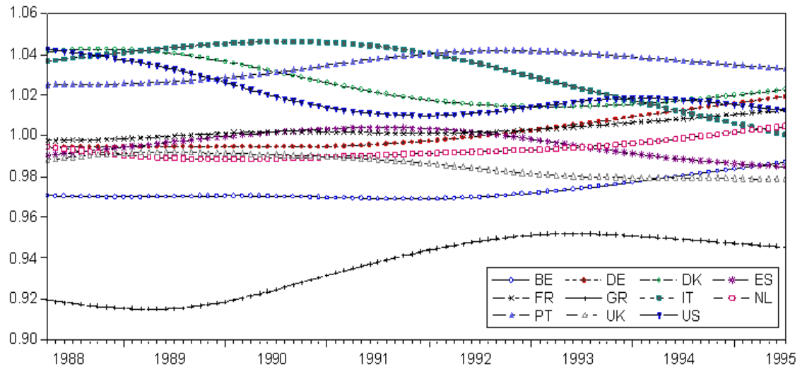
Figure 4: h_{ict} for the U.S. dollar price of i =fuel for each of 11 countries
