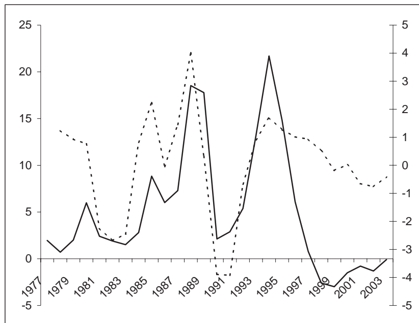
Figure 2. RPI Inflation Rate vs Output Gap
