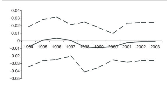
Coefficient of Lagged Inflation \pm 2 SE
