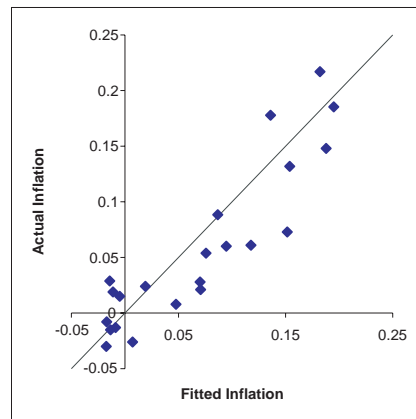
Figure 4. Actual Inflation and Fit of Hybrid NKPC
